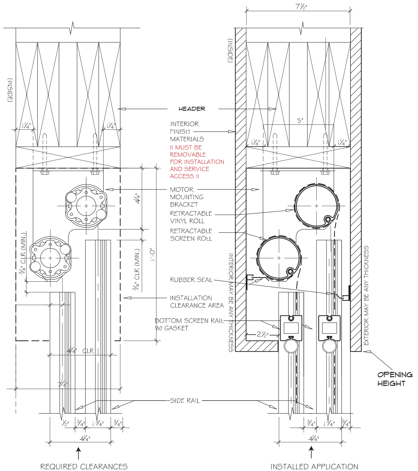
2B CROSS SECTION - DOUBLE ROLLER - UNDER HEADER MOUNT 3" = 1'-0"
